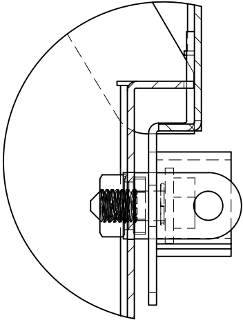
DETAIL L SCALE 1:2
